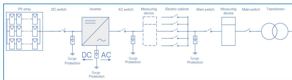
Schematic of a central inverter PV system (no microinverters or dc-to-dc converters (optimizers), and multiple arrays connected to the inverter) connected to a public utility power grid. (Source: ZRS)
