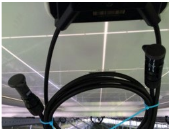
Example of a PV modules with unmatted connectors with protective caps (Picture/Illustration of Stäubli, Switzerland)
