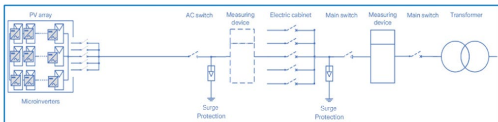
Schematic of a PV system with microinverters connected to a public utility power grid. (Source: ZRS)
