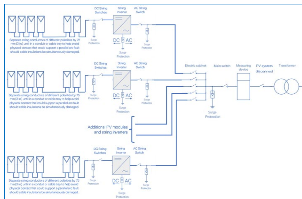
Schematic of a string inverter system (no microinverters and no dc-to-dc converters (optimizers)) with one array connected to each inveter. All inverters are connected to a public utility grid. (Source: ZRS)
