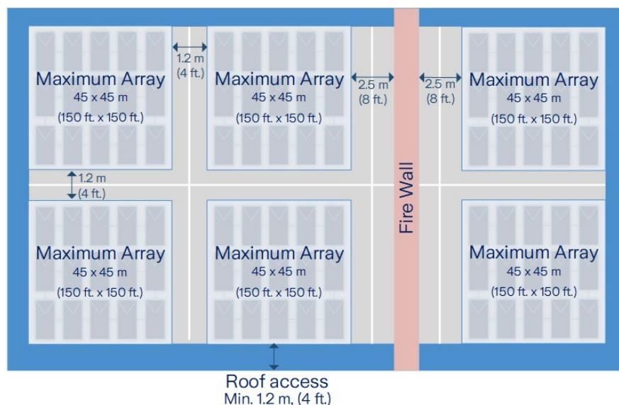
Rooftop diagram depicting the separation of a firewall from PV arrays. It also shows the PV array roof edge setback, maximum array size, and minimum array spacing. (Source: ZRS)
