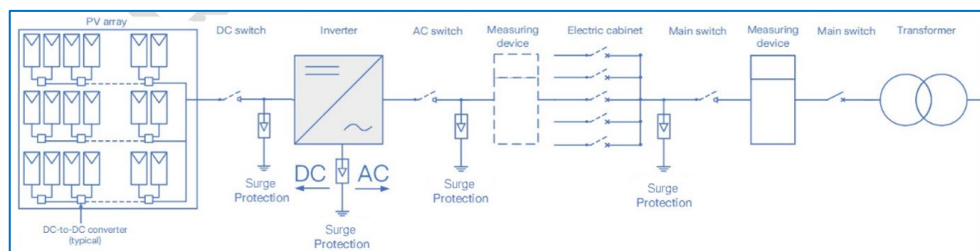
Schematic of a PV system with dc-to-dc converters (optimizers) connected to a public utility power grid. (Source: ZRS)
