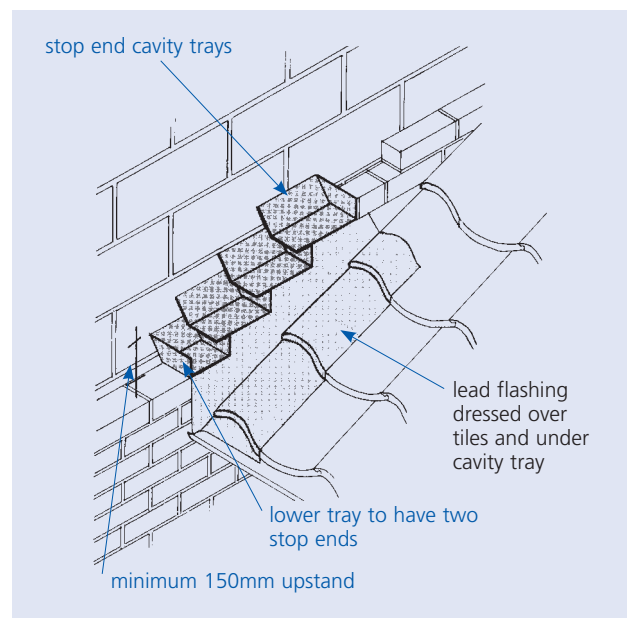
Stepped cavity tray detail at roof/cavity wall abutment
