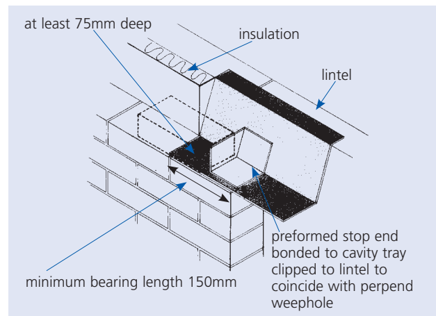
Stop end
