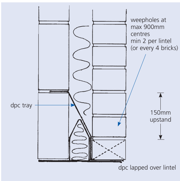
Typical cavity tray installation
