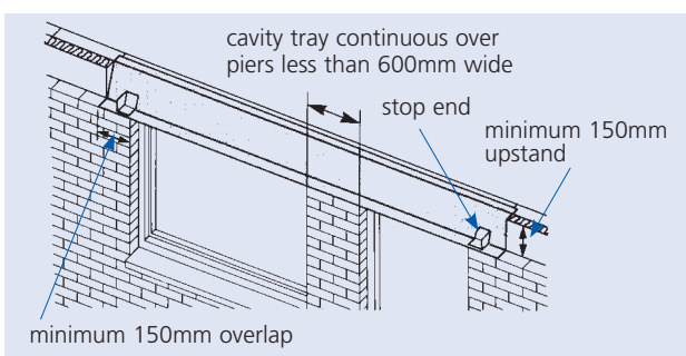
Cavity tray continuous over a pier
